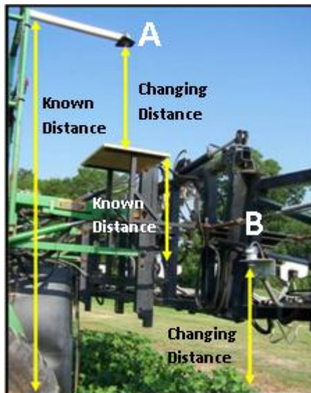
Figure 3. Ultrasonic height sensor A measures height of the boom and height sensor B measures the distance from the sensor to the plant. Using a set distance from sensor A to the ground and sensor B to the top of the boom, plant height can be calculated.
